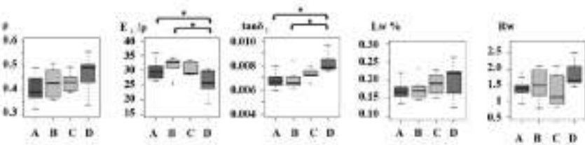
Fig.2 Distribution of some physical-mechanical properties and optical features of resonance spruce plates according to different quality grades (A=highest, D=lowest): the significance of differences between grades is indicated by a star (*).
