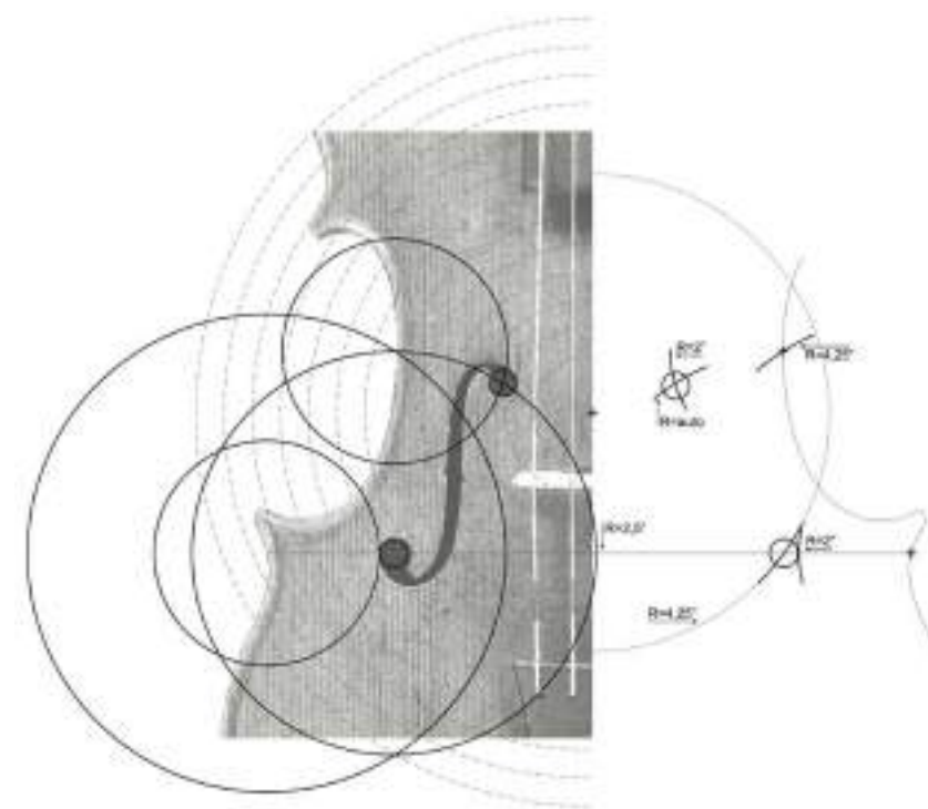
Viol by Girolamo Amati [8], showing the construction of the f-holes according to the sketches of A. Stradivari; all values in Roman oncia.
